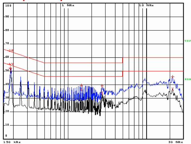
18W/12-24v/78AL
