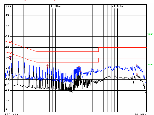
36W/12-24v/78AL
